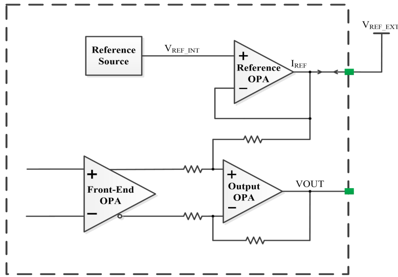
Reference output function circuit
