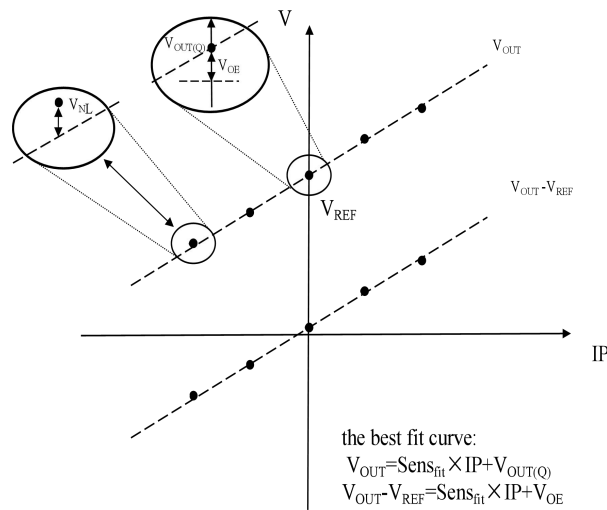
Output vs IP
