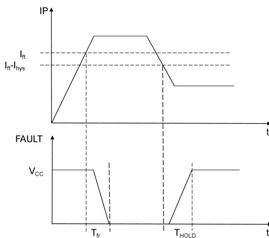
Overcurrent Fault Timing Diagram
