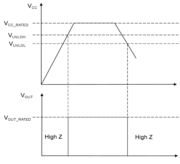
UVLO Timing Diagram
