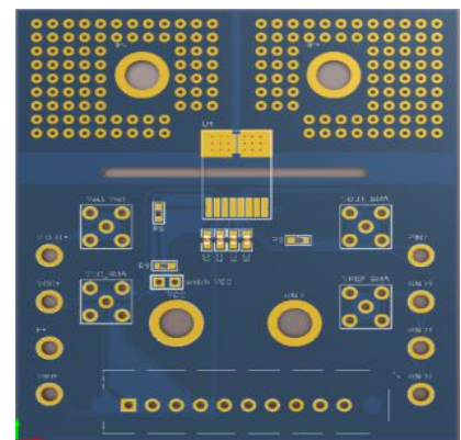
NHC3001 Demo Board
