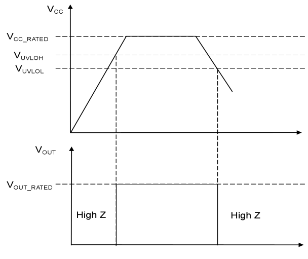
Under-Voltage Protection Timing Diagram
