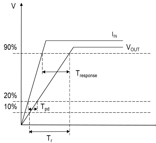
Output Response
