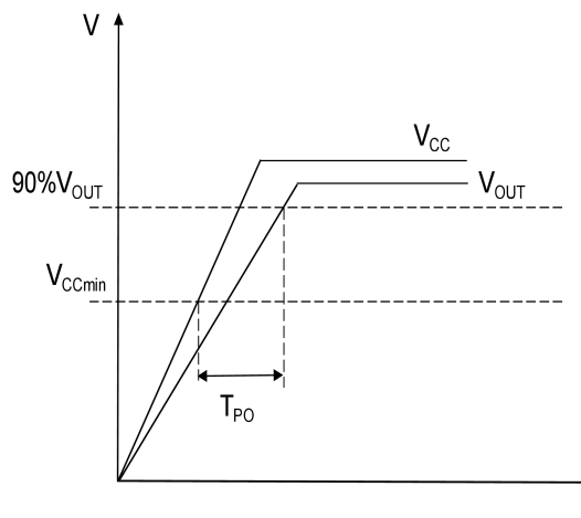
Power-on Reset
